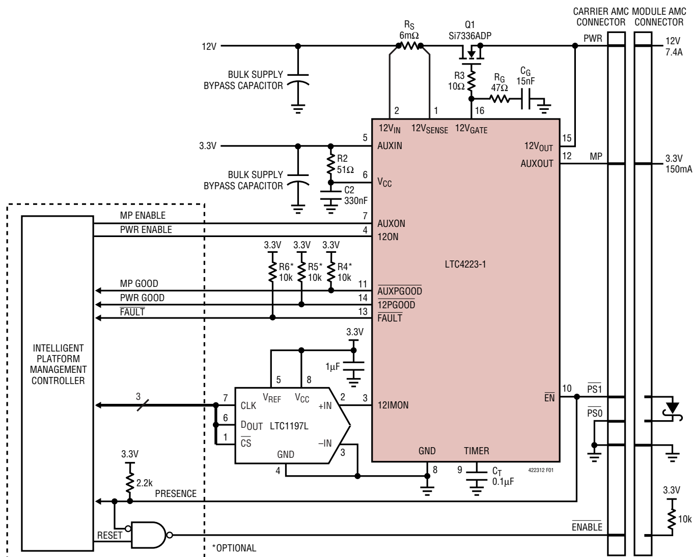
Figure 1. Advanced Mezzanine Card/MicroTCA Application
