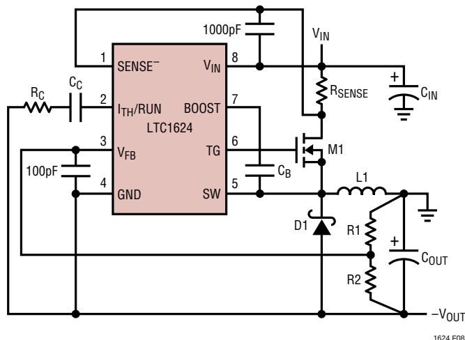
Figure 8. Positive-to-Negative Converter
