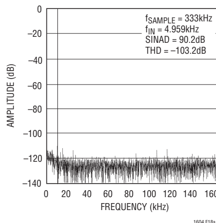
Figure 18a. This FFT of the LTC1604's Conversion of a Full-Scale 5kHz Sine Wave Shows Outstanding Response with a Very Low Noise Floor When Sampling at 333kps
