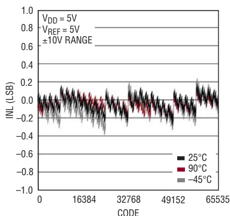
LTC2753-16 Integral Nonlinearity (INL)
