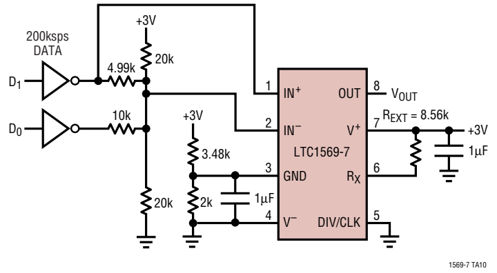
Pulse Shaping Circuit for Single 3V Operation, 400kbps (200ksps) 4 Level Data, 128kHz Cutoff Filter
