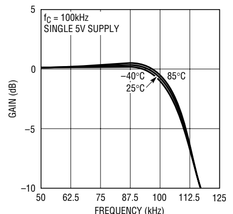
Roll-Offs Over Temperature ( f_C = 100\text{kHz} )
