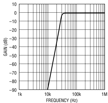
Amplitude Response
