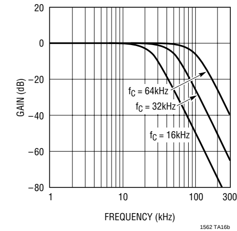
Amplitude Response
