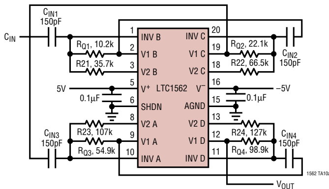
8th Order Highpass 0.05dB Ripple Chebyshev Filter f_{\text{CUTOFF}} = 30\text{kHz}
