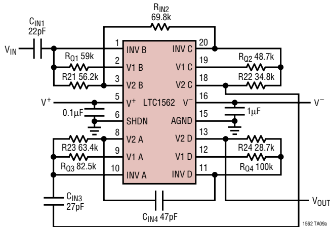
8th Order Wideband Bandpass Filter f_{\text{CENTER}} = 50\text{kHz} , -3\text{dB BW } 40\text{kHz to } 60\text{kHz}
