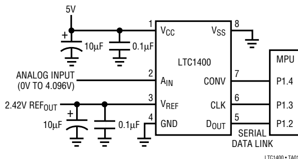
Single 5V Supply, 400kHz, 12-Bit Sampling A/D Converter
