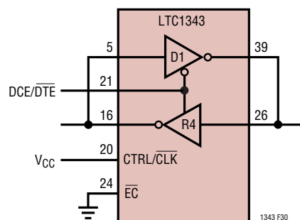
Figure 30. Single-Ended Driver and Receiver Enable
