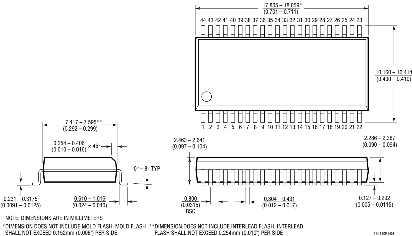
GW Package 44-Lead Plastic SSOP (Wide 0.300) (LTC DWG # 05-08-1642)
