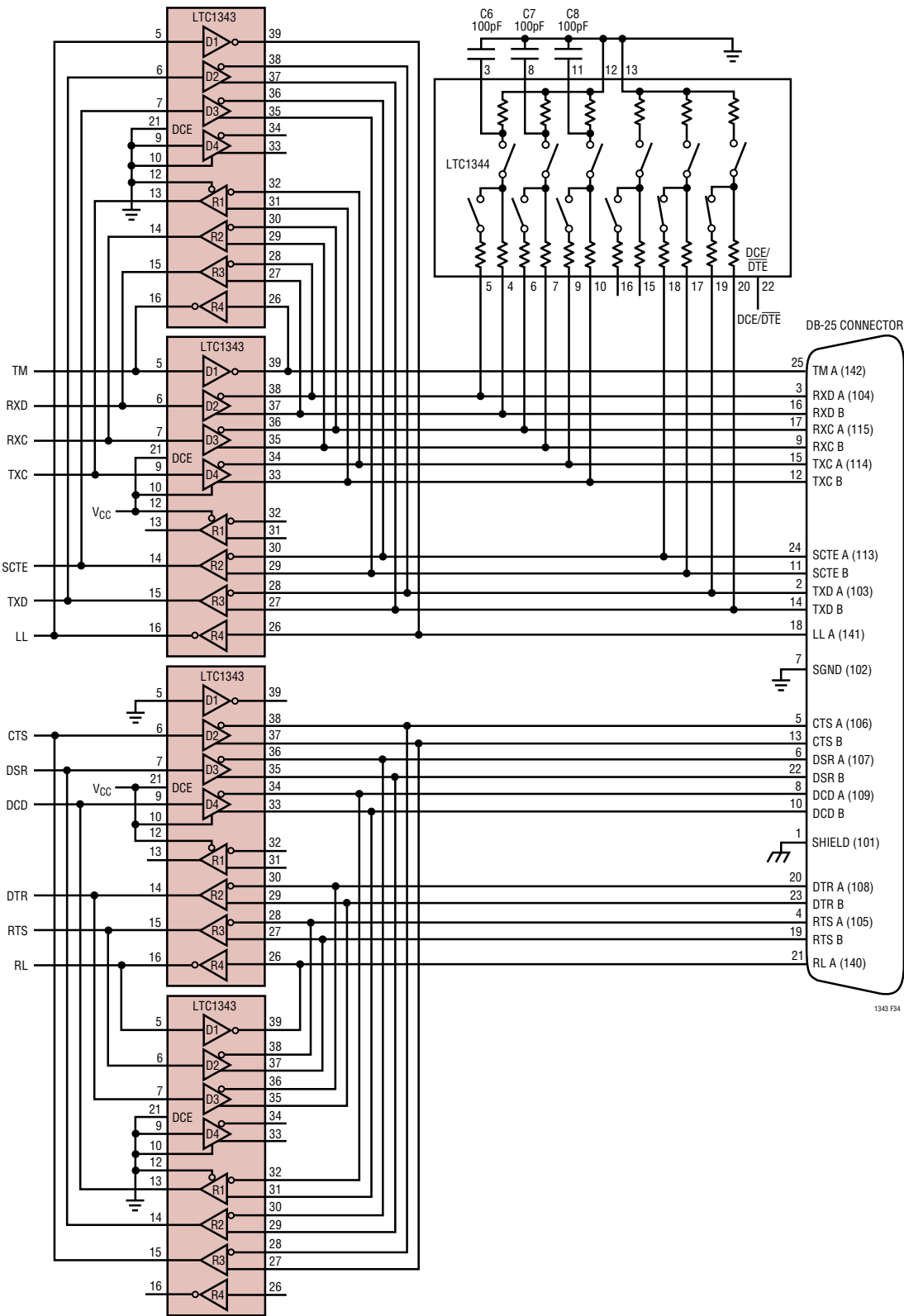
Figure 34. Controller-Selectable Multiprotocol DTE/DCE Port with DB-25
