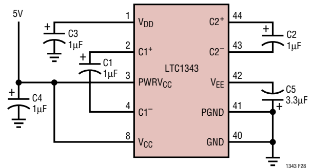
Figure 28. Charge Pump
