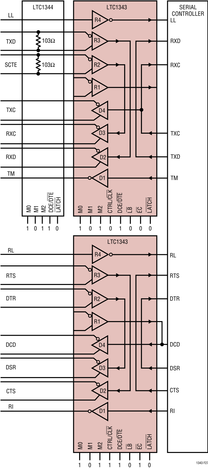
Figure 27. Echoed Clock, DCE Loop-Back
