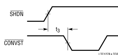
\overline{SHDN} to \overline{CONVST} Wake-Up Timing
