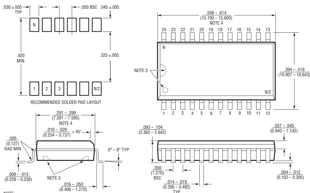
SW Package 24-Lead Plastic Small Outline (Wide .300 Inch) (Reference LTC DWG # 05-08-1620)
