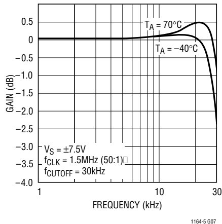
Maximum Passband over Temperature for V_S = \pm 7.5V , 50:1
