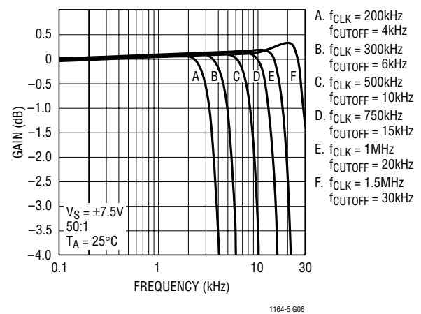
Passband vs Frequency and f_{CLK}
