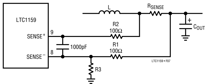
Figure 7. Suppressing Burst Mode Operation
