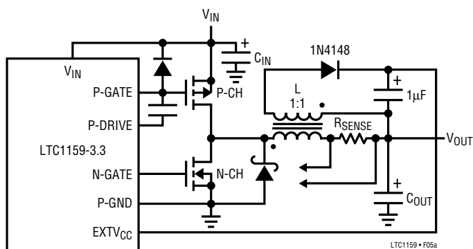
Figure 5a. Inductive Boost Circuit for EXTV_{CC}
