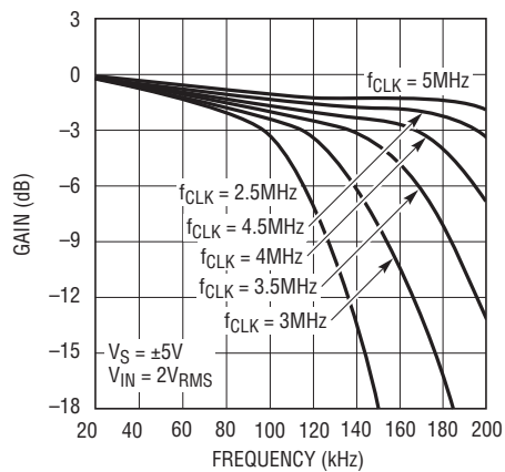
Passband Gain vs Clock Frequency
