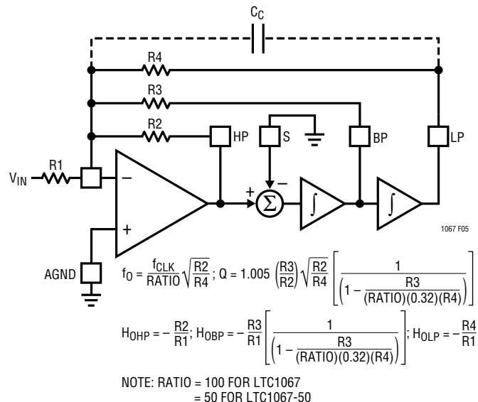
Figure 5. Mode 3, 2nd Order Section Providing Highpass, Bandpass and Lowpass Outputs
