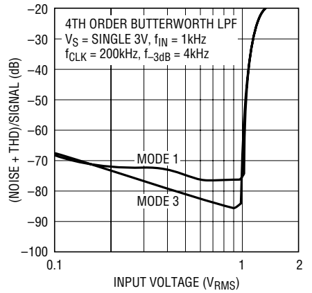
LTC1067-50 Noise + THD vs Input Voltage
