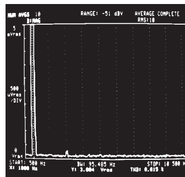
Harmonic Distortion, 8th Order LP Butterworth, f_C = 20\text{kHz} , THD = 0.015% for 3V_{\text{RMS}} Input
