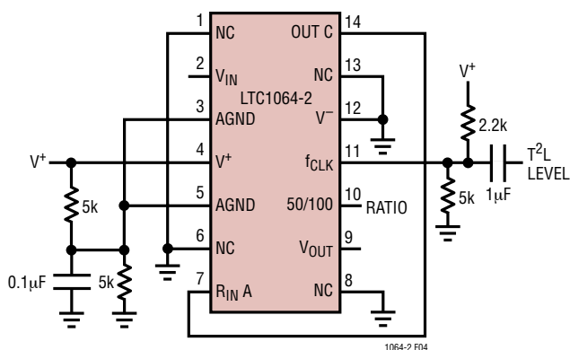
Figure 4. Level Shifting the Input T 2 L Clock for Single Supply Operation \geq 6V .
