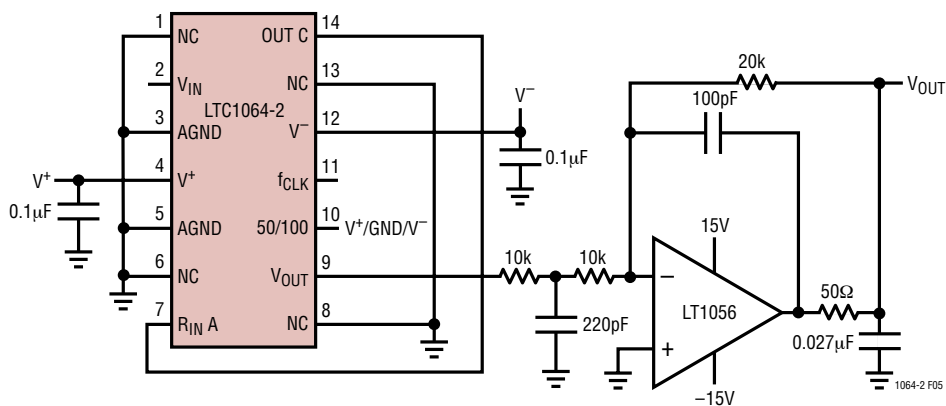
Figure 5. Adding an Output Buffer-Filter to Eliminate Any Clock Feedthrough. Passband \pm 0.1\text{dB} to 50kHz, -3\text{dB} at 94kHz.
