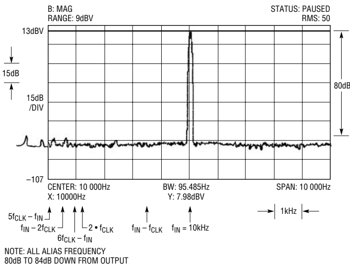
Figure 6b. Output Voltage Spectrum of 1/2 LTC1051 Operating as a Unity-Gain Inverting Amplifier. V_S = \pm 5\text{V} , R_L = 10\text{k}\Omega , C_L = 50\text{pF} , V_{IN} = 8\text{V}_{\text{P-P}} , 10\text{kHz}
