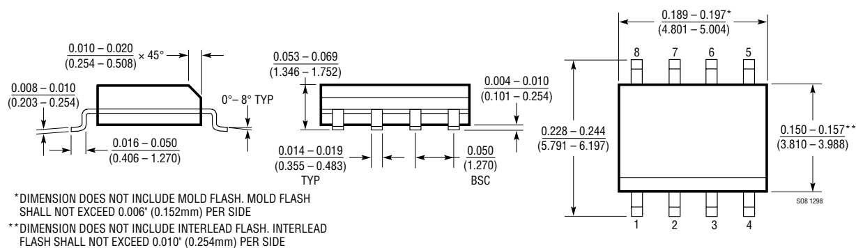
S8 Package 8-Lead Plastic Small Outline (Narrow .150 Inch) (Reference LTC DWG # 05-08-1610)
