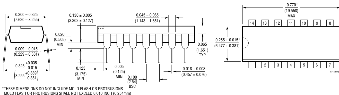
N Package 14-Lead PDIP (Narrow .300 Inch) (Reference LTC DWG # 05-08-1510)
