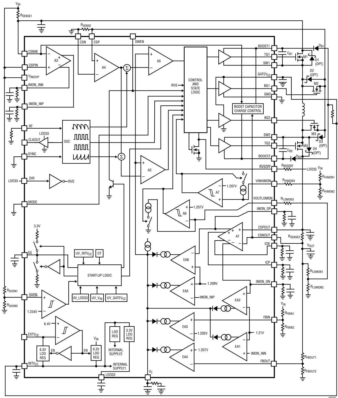
Figure 1. Block Diagram
