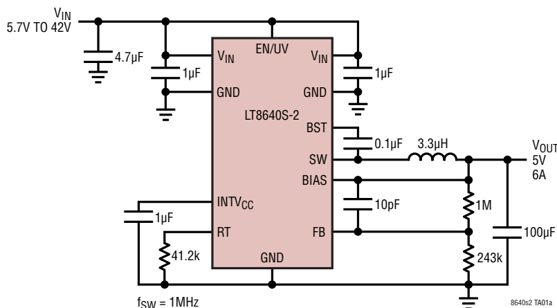
5V, 6A Step-Down Converter
