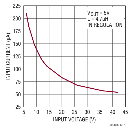
LT8643S-2 No-Load Supply Current
