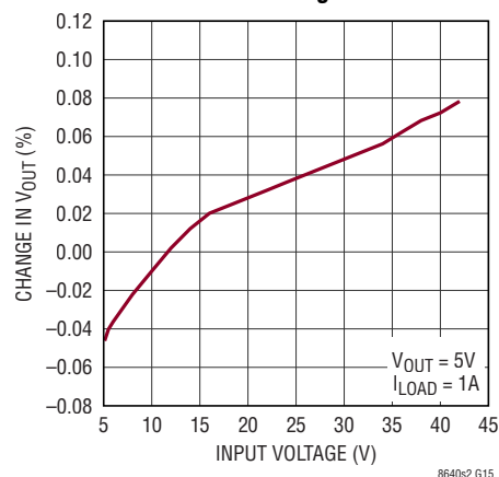
LT8640S-2 Line Regulation
