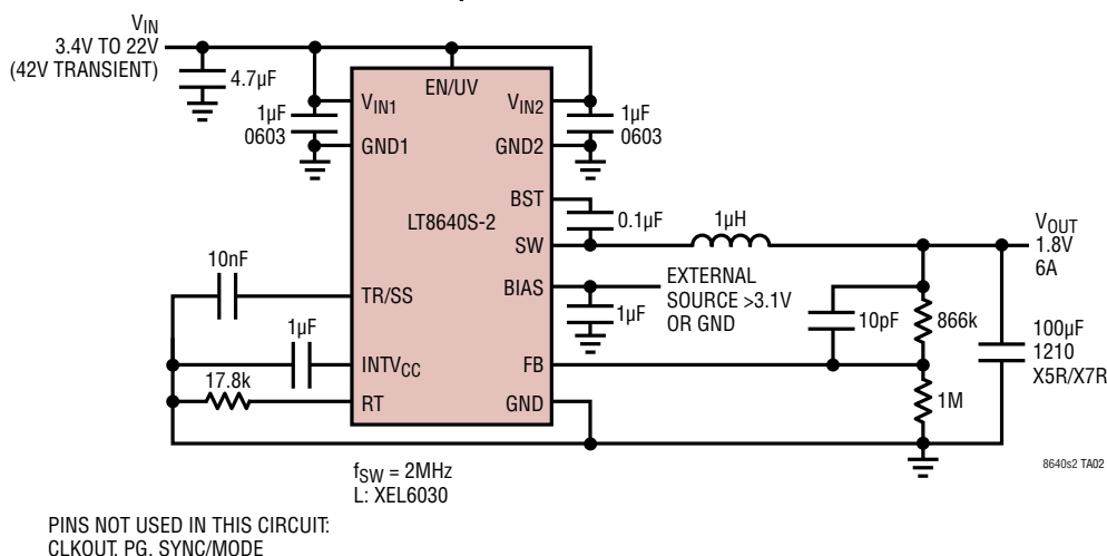
2MHz 1.8V, 6A Step-Down Converter
