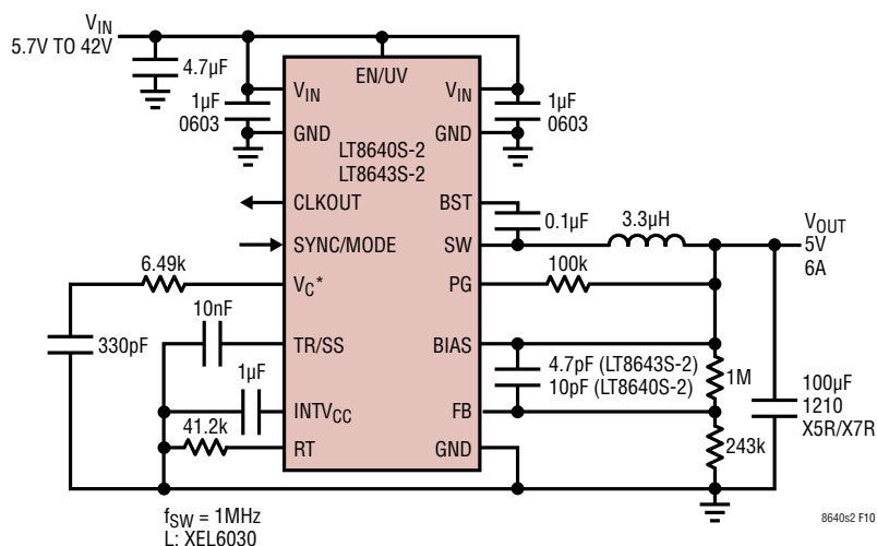
Figure 10. 5V, 6A Step-Down Converter with Soft-Start and Power Good
