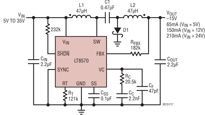
Figure 17. Dual Inductor Inverting Converter: The Component Values Given Are Typical Values for a 700kHz 5V-35V to -15V Inverting Topology Using Coupled Inductors
