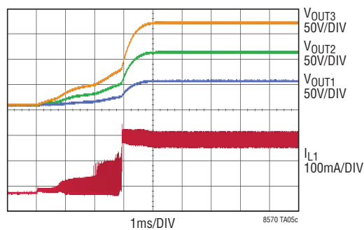
Start-Up Waveforms
