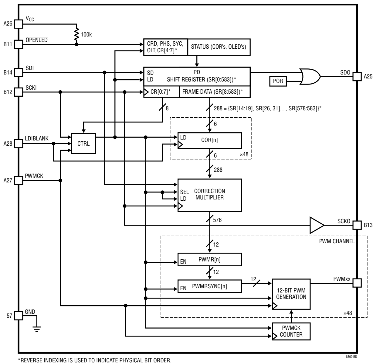
Figure 1. Block Diagram
