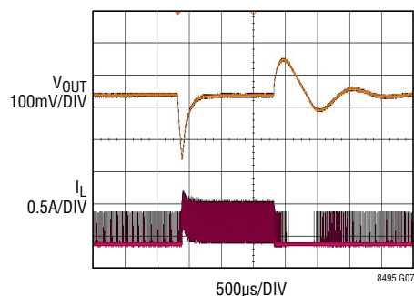
Transient Load Response; Load Current Is Stepped from 20mA (Burst Mode Operation) to 220mA
