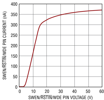
SWEN/ \overline{\text{RSTIN}} /WDE Pin Current
