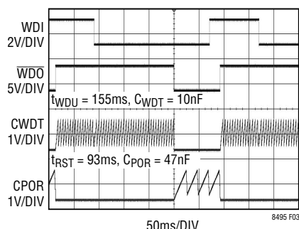
Figure 3. Timeout Watchdog Waveforms
