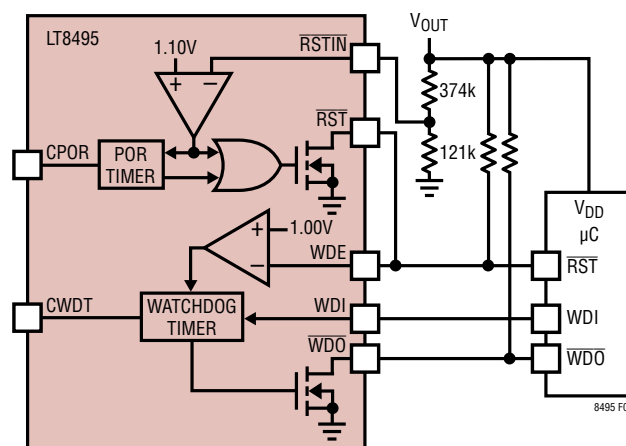
Figure 7. Watchdog Monitoring
