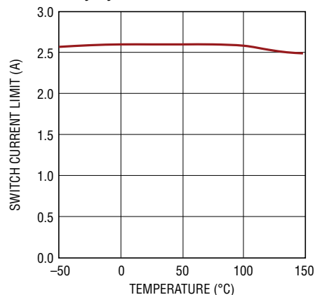
Switch Current Limit at Minimum Duty Cycle
