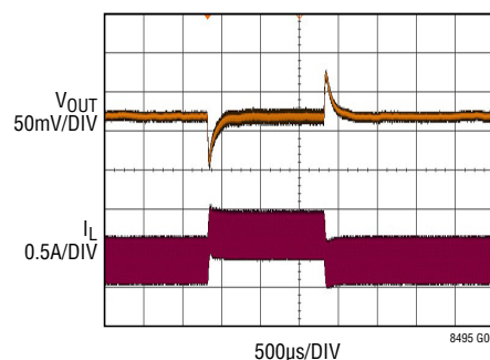
Transient Load Response; Load Current Is Stepped from 300mA to 500mA
