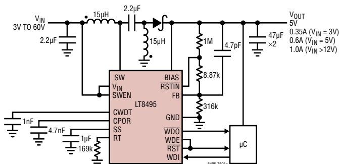
450kHz, 5V Output SEPIC Converter
