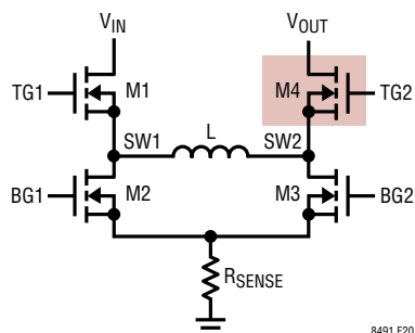
Figure 20. Simplified Diagram of Power Switches
