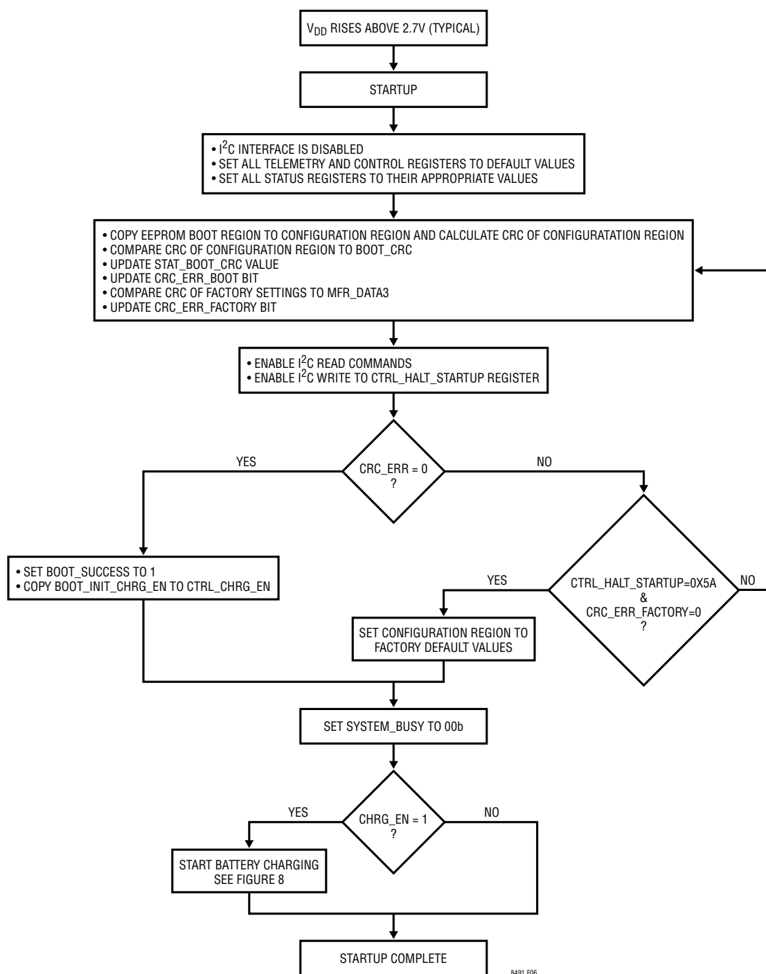
Figure 6. Startup Sequence
