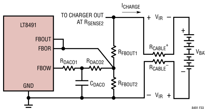
Figure 33. IR Drop Present in Battery Connection
