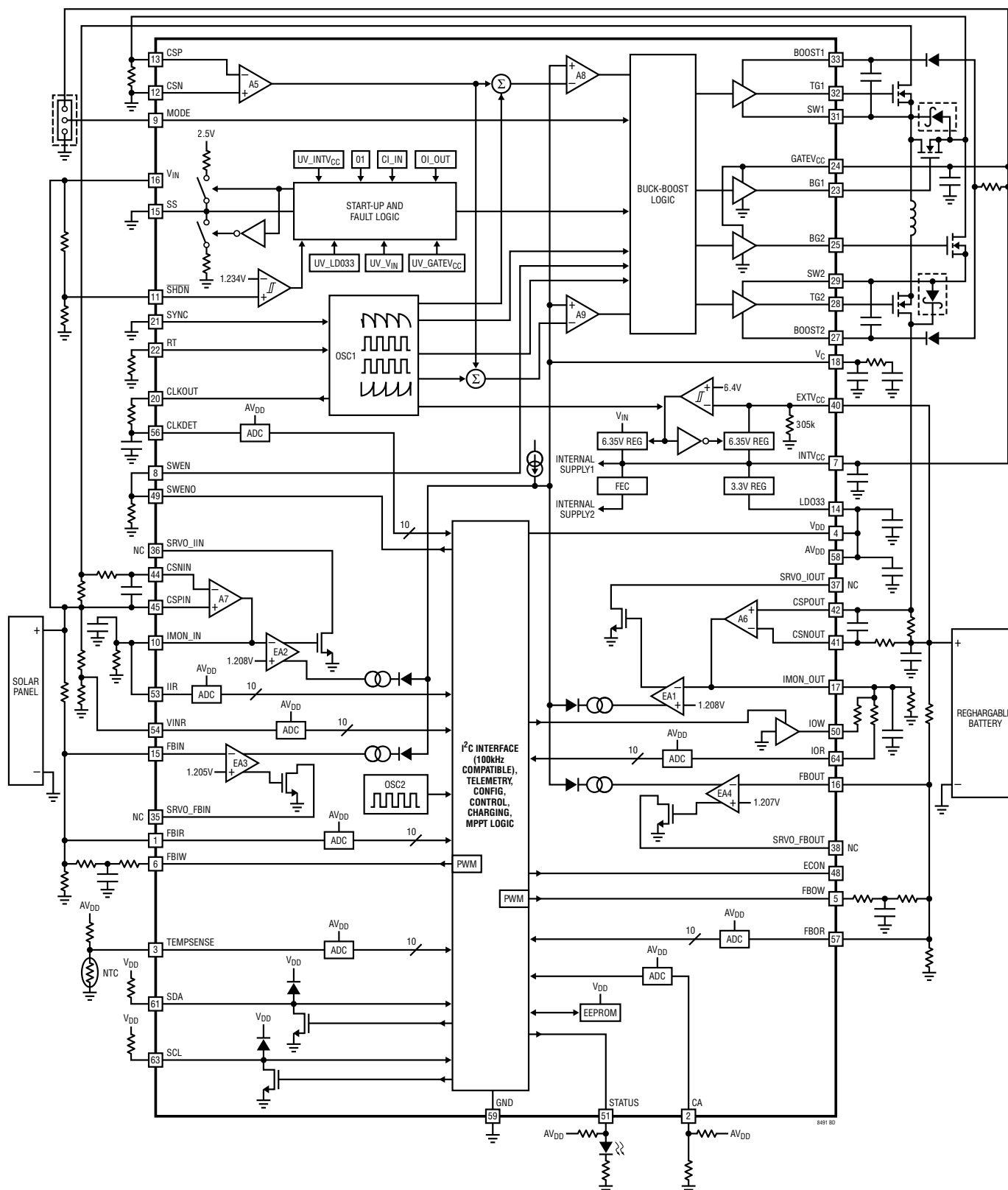
Figure 1. Block Diagram
