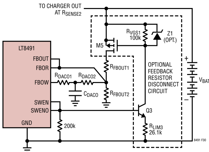
Figure 30. Optional Feedback Resistor Disconnect Circuit #1
