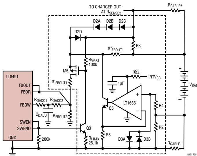
Figure 35. How to Combine Figure 30 and Figure 34
