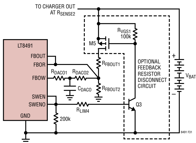
Figure 31. Optional Feedback Resistor Disconnect Circuit #2
