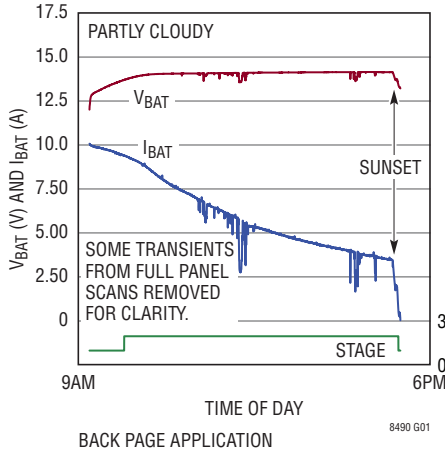
Solar Powered Charging Lead Acid Battery "A"
