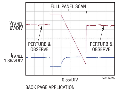
Maximum Power Point Tracking
