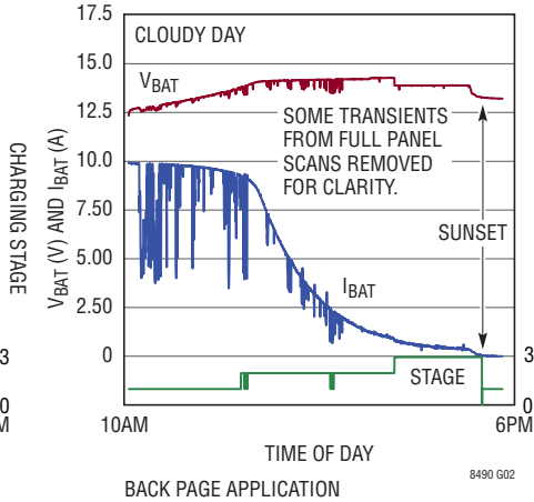
Solar Powered Charging Lead Acid Battery "B"
