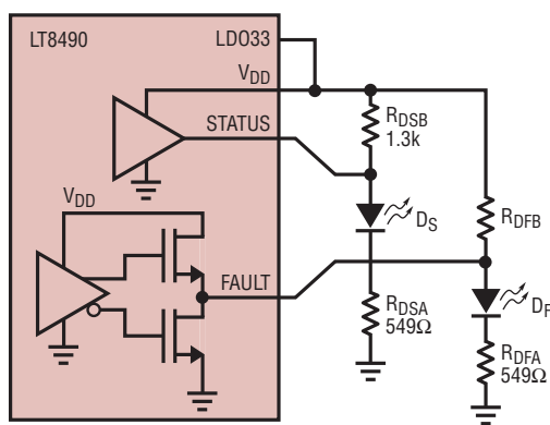
D_S : OSRAM, LGL29KF2J124Z D_F : OSRAM, LGL29K-H1J2-1-Z
