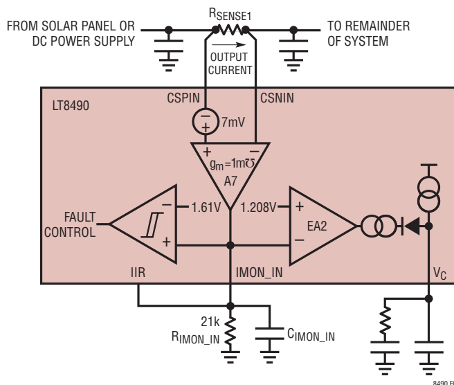
Figure 9. Input Current Regulation Loop
