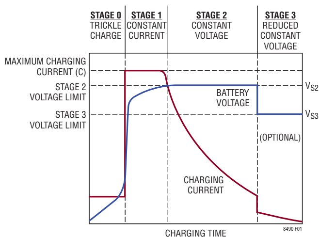
Figure 2. Typical Battery Charging Cycle
