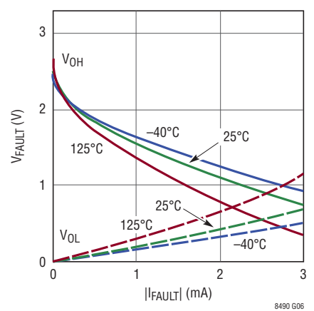
FAULT V_{OH} and V_{OL} ( V_{DD} = AV_{DD} = 3.3V )
