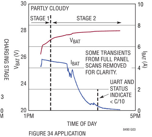
Solar Powered Charging Lithium Ion Battery
