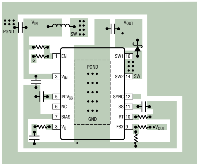
(a) MSOP
