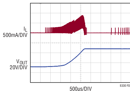
Figure 3. Soft-Start Waveforms
