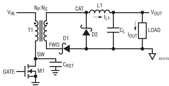
Figure 3. Forward Converter Architecture (Nonsynchronous)
