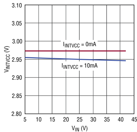
INTV CC Voltage vs V_{\text{IN}}
