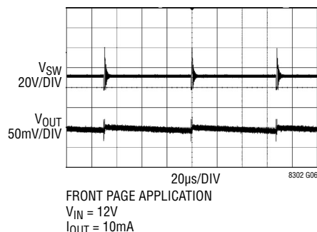
Burst Mode Waveforms
