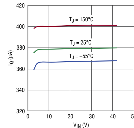
V_{IN} Quiescent Current, Active Mode
