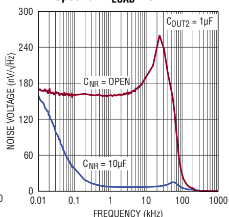
2.5V V_{OUT2} Output Voltage Noise Spectrum I_{LOAD} = 0\text{mA}
