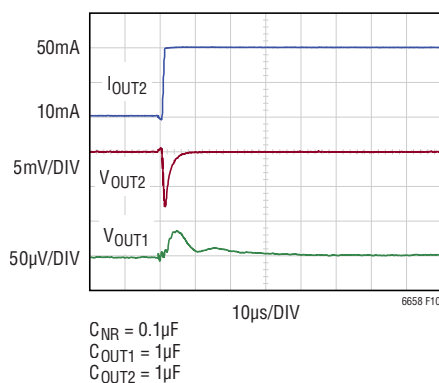
Figure 10. LT6658-2.5 Output 2 Response to 40mA Load Step
