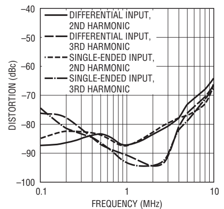
Distortion vs Frequency V_IN = 2V_P-P, V_S = ±5V, R_L = 800Ω at Each Output, T_A = 25°C, Gain = 1
