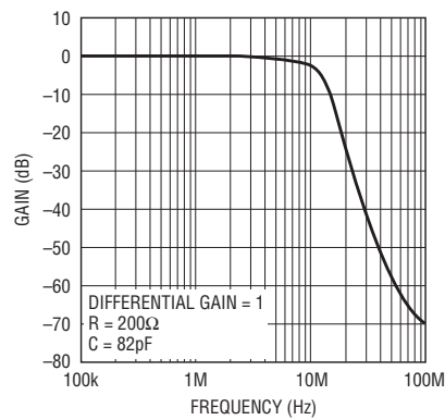
Amplitude Response
