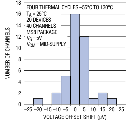
Voltage Offset Shift vs Thermal Cycling
