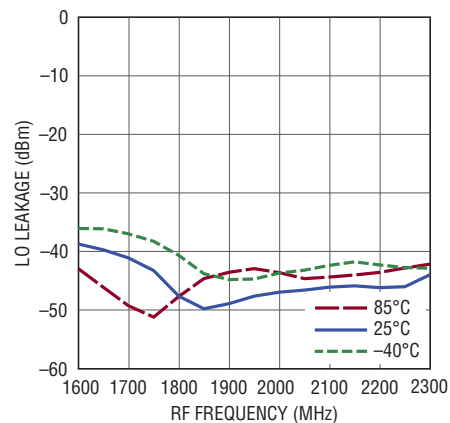
LO-RF Leakage vs RF Output Frequency
