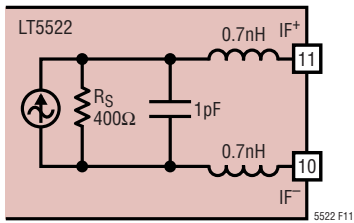
Figure 11. IF Output Small-Signal Model
