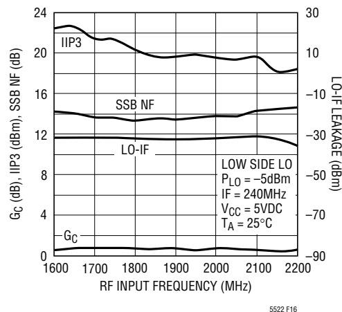
Figure 16. Typical Performance Using a Narrowband Bridge Balun (Swept RF)
