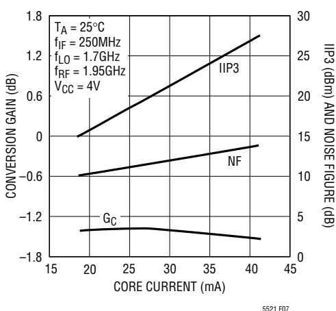
Figure 7. IIP3, G C and Noise Figure vs Core Current, Constant Supply Voltage
