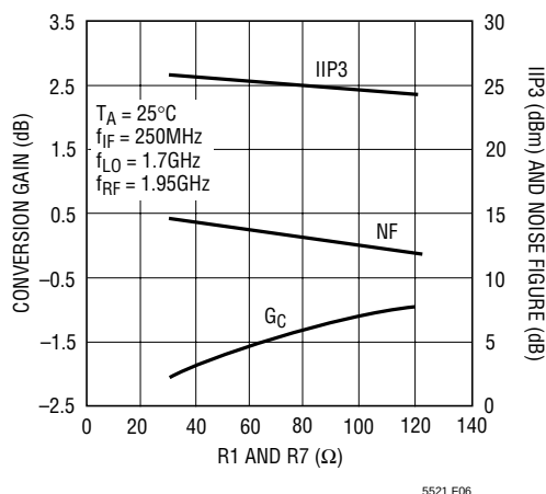
Figure 6. IIP3, G C and Noise Figure vs External Resistance, Constant Core Current (Variable Supply Voltage)
