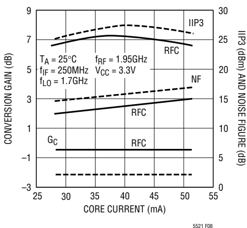
Figure 8. Comparison of 3.3V Performance With and Without Input RF Choke
