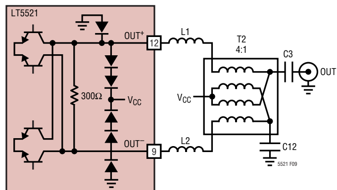
Figure 9. Simplified Output Circuit with External Matching Components
