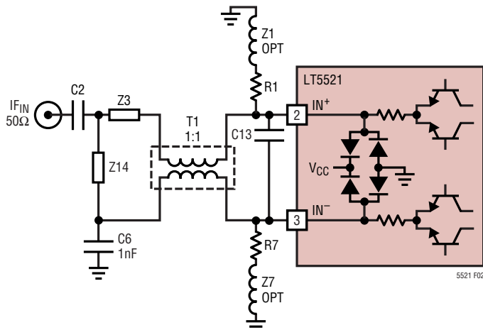
Figure 2. Signal Input with External Matching
