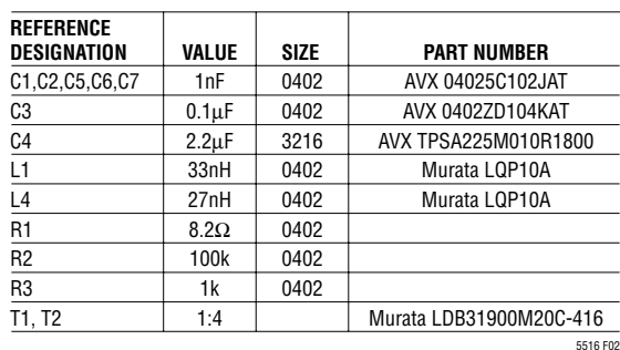
Figure 2. 900MHz Evaluation Circuit Schematic
