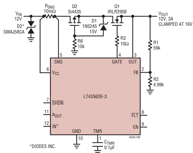
Figure 8. Overvoltage Regulator with P-Channel MOSFET Reverse Input Protection
