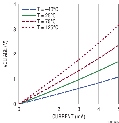
PWRGD, \overline{T2P} Output Low Voltage vs Current
