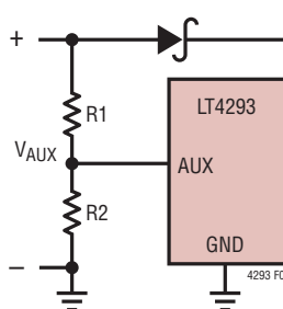
Figure 7. AUX Threshold and Hysteresis Calculation
