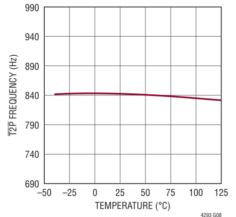
\overline{T2P} Frequency
