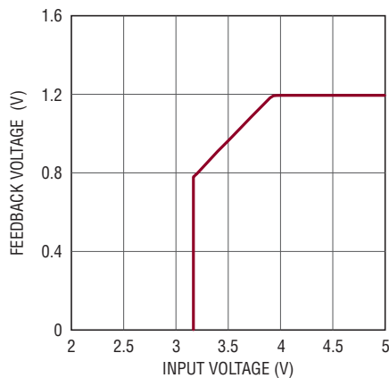
Feedback Regulation Voltage
