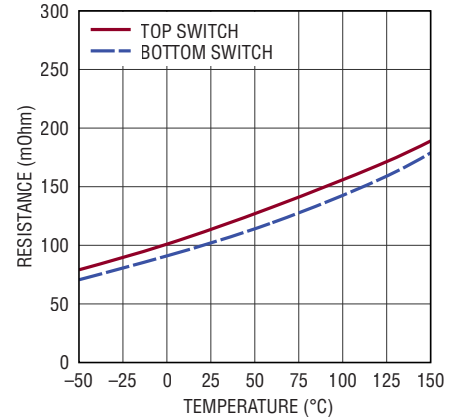
Power Switch On-Resistance
