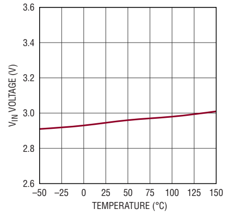
V_{IN} UVLO Threshold (Rising)
