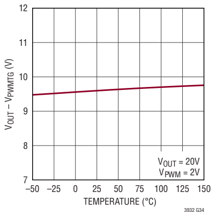
PWMTG Voltage
