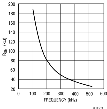
Figure 1. Timing Resistor ( R_{SET} ) Value
