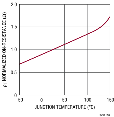
Figure 10. Normalized R_{DS(ON)} vs Temperature
