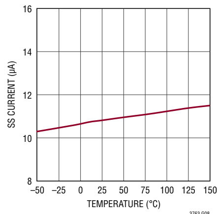
SS Current
