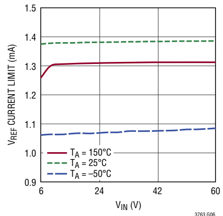
VREF Current Limit
