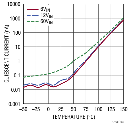
Quiescent Current (Shutdown)
