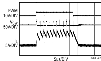
PWM Dimming
