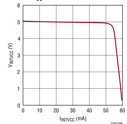
INTVCC Current Limit
