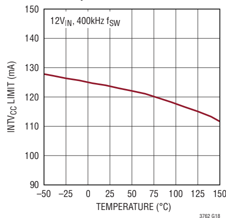
INTV CC Maximum Source Current vs Temperature
