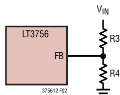
Figure 2. Feedback Resistor Connection for Boost or SEPIC LED Drivers
