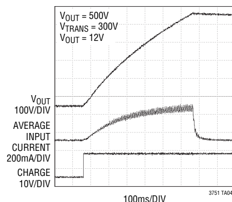
Charging Waveform
