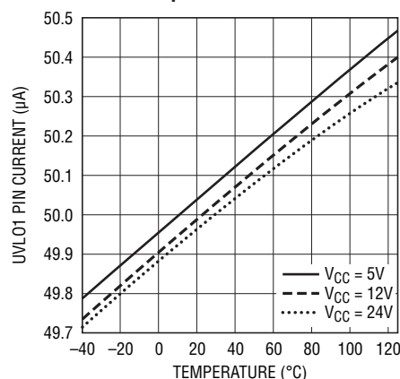
UVL01 Trip Current
