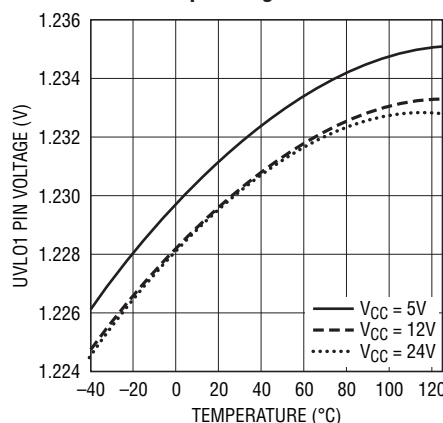
UVL01 Trip Voltage
