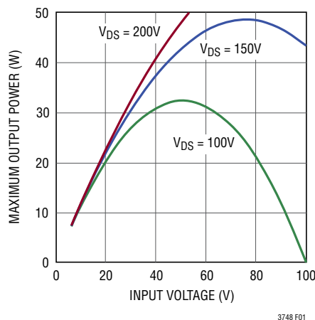
Figure 1. Maximum Output Power at 12V OUT with a 3A I_{LIM} and Maximum V_{DS} = 100\text{V}, 150\text{V}, 200\text{V}
